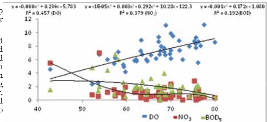
Figure 4: Polynomial fit of WQI (NSF) for the WQ data from 2003-2012
