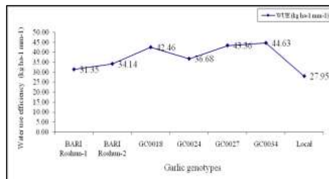
Fig.2: Water use efficiency of garlic genotypes on an average of two years
