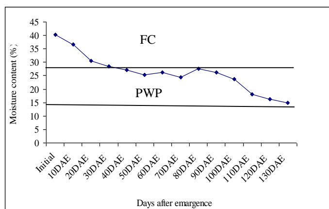
Fig.1: Soil moisture level at ten days interval on an average of two years [FC= Field capacity, PWP= Permanent wilting point]
