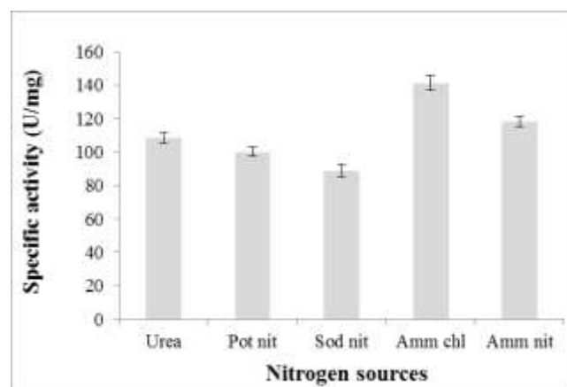
Fig. 3(a, b, c): Alkaline protease activity of strain Bacillus licheniformis HSW-16 under different salt concentrations, carbon and nitrogen sources.
