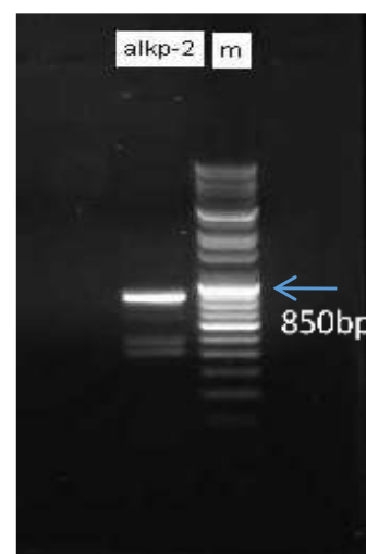
Fig 1: Amplified gel image of alkaline protease gene of Bacillus licheniformis . Lane M denotes the Marker, Lane alk: amplified alkaline protease gene of isolate HSW-16
