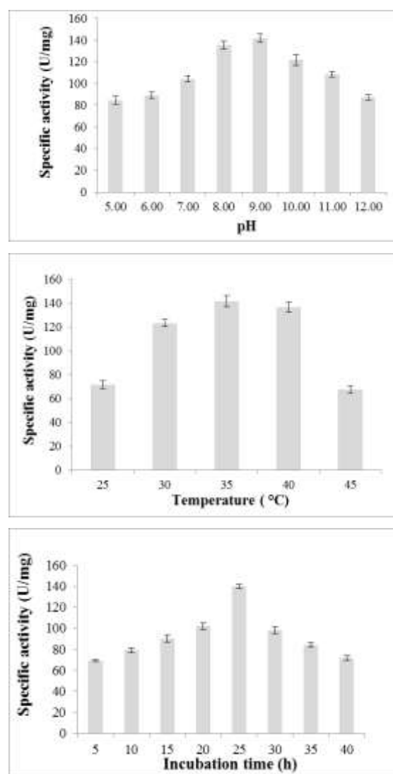
Fig 2(a, b, c): Effect of varying pH, temperature and incubation time on activity of alkaline protease of Bacillus licheniformis HSW-16.
