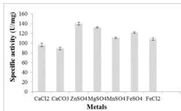
Fig. 4: Effect of various metal ions on protease activity of isolate Bacillus licheniformis HSW-16.
