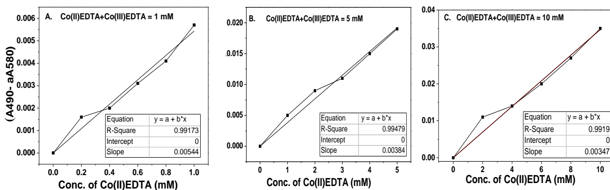
Fig. 2: Calibration curves of 0-1, 0-5 and 0-10 mM of Co(II)EDTA.
