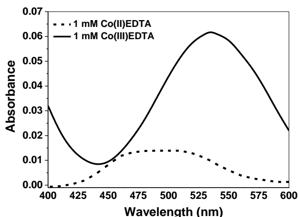
Fig. 1: Absorption spectrum of Co(II)EDTA and Co(III)EDTA in the visible range.
