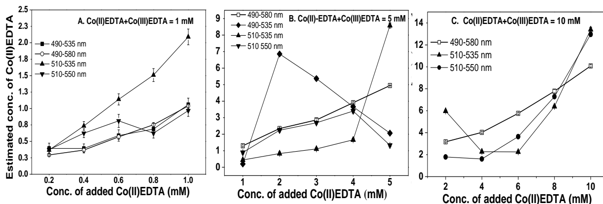
Fig. 3: Comparison of estimated concentration of Co(II)EDTA using the wavelength pair 490-580 nm and the actual concentration of Co(II)EDTA.
