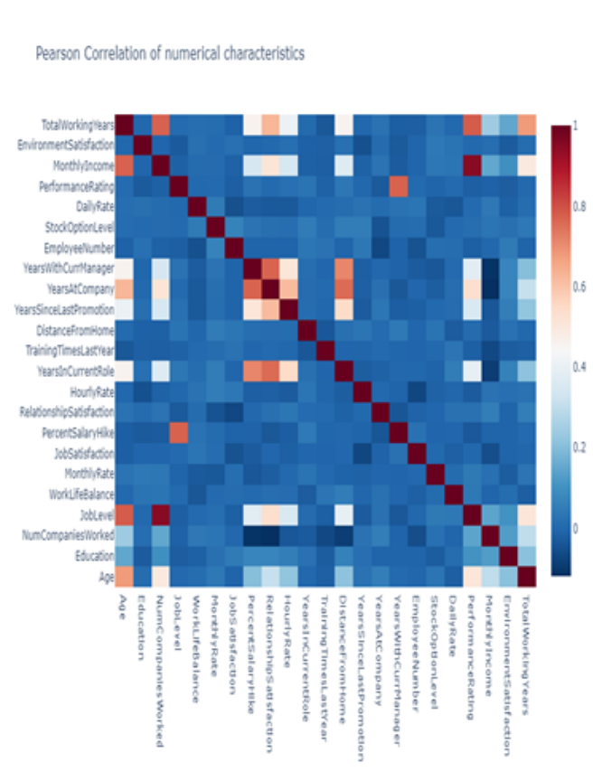
Fig. 3. Person correlation of numerical characteristics
