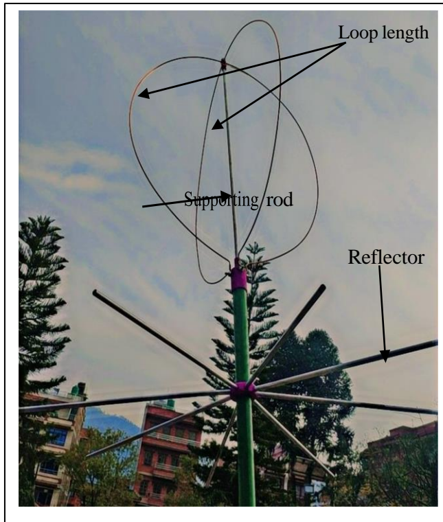
Fig. 2. Standard Eggbeater Antenna
