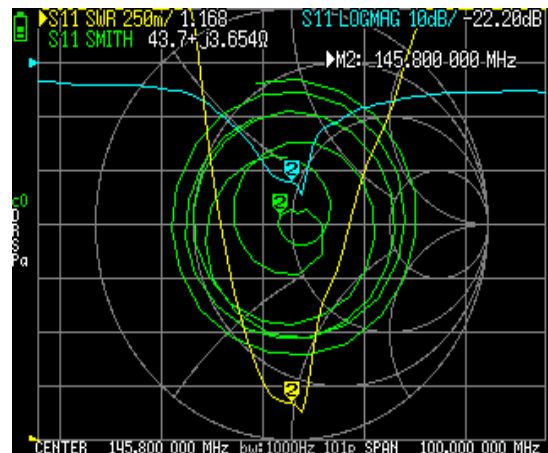
Fig. 3. NANO VNA test result of eggbeater antenna
