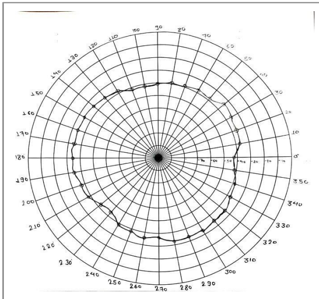
Fig. 4. Radiation pattern of eggbeater antenna
