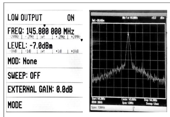
Fig. 6. Output appears when signal is on
