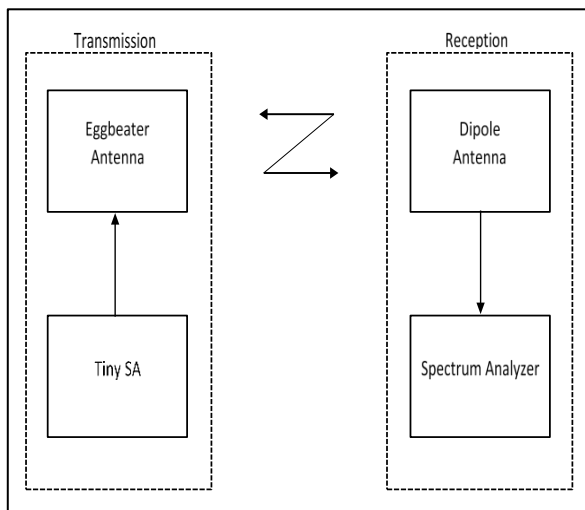
Fig. 1. Block diagram of system model
