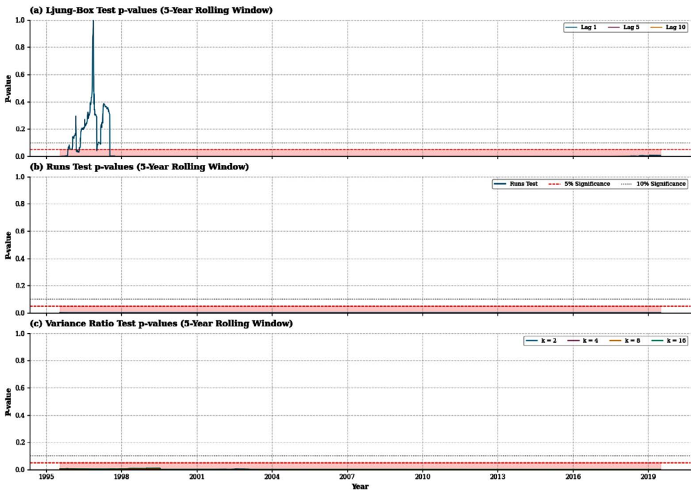
Figure 2: Linear Efficiency Test p-values using 5-Year Rolling Window
